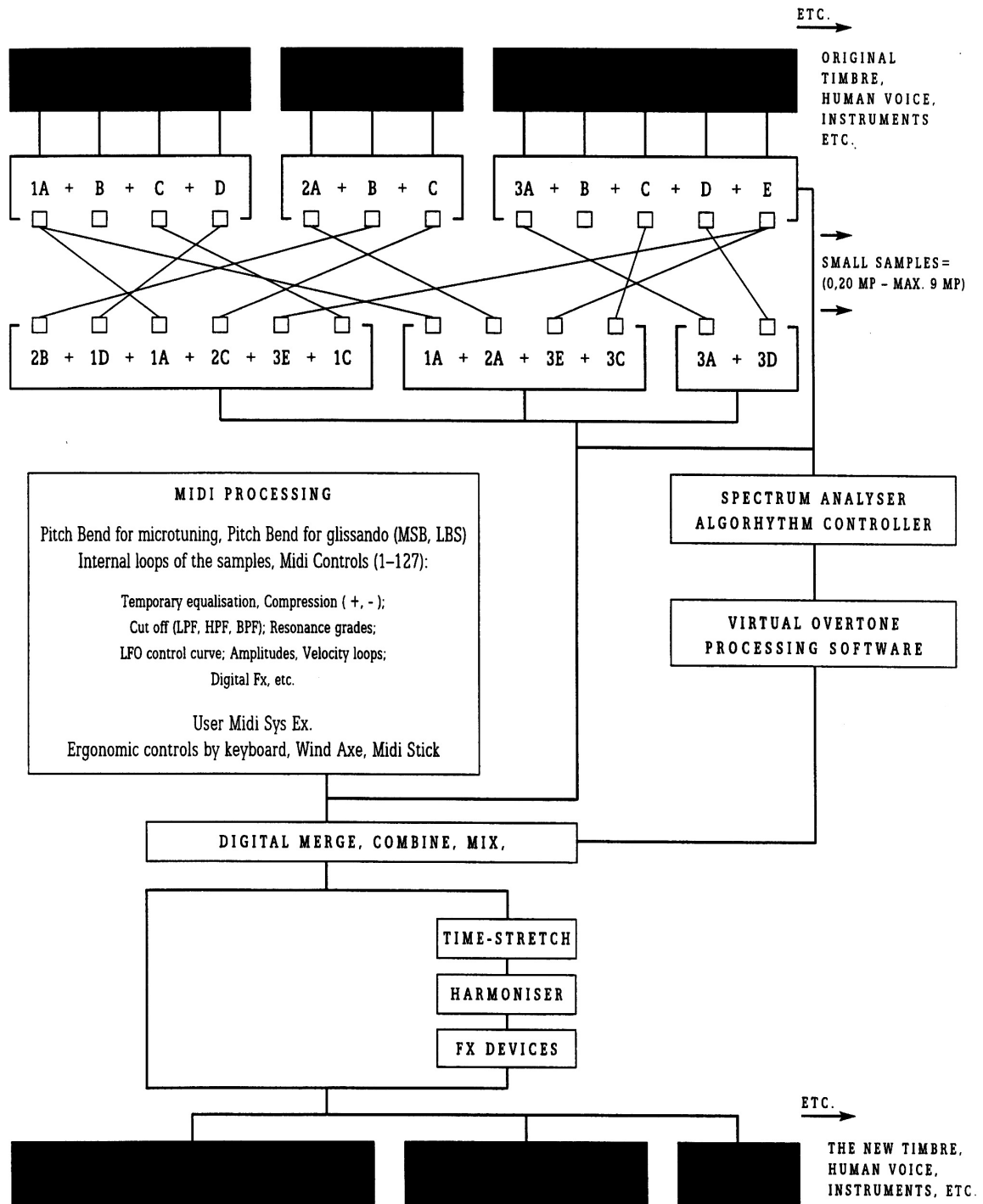
System Block Diagram of the virtual timbres in eL-Hortobāgyi 'music
